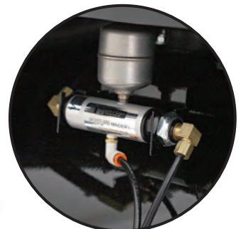
Tank drain automatically drains liquid from air receiver
